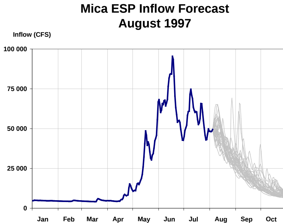
Figure 1 Series of synthetic hydrographs produced using the ESP forecasting procedure. Forecast date is 01 August in the example
