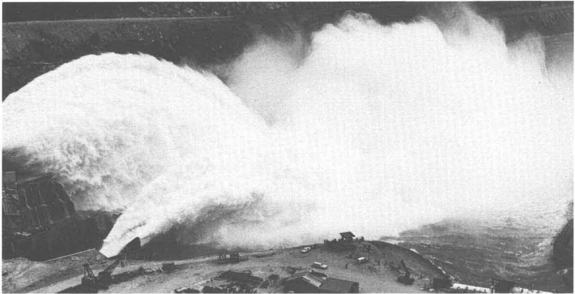
MICA DAM Spillway and outlet works in operation.
