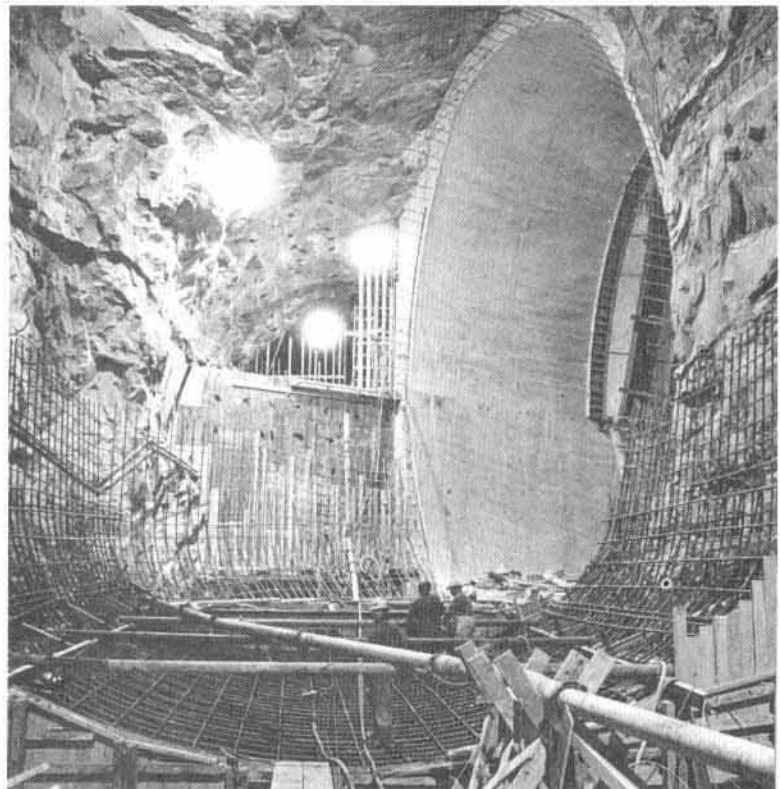
TAILRACE MANIFOLD No. 2 and draft tube for Unit No. 6 at Mica powerhouse.
