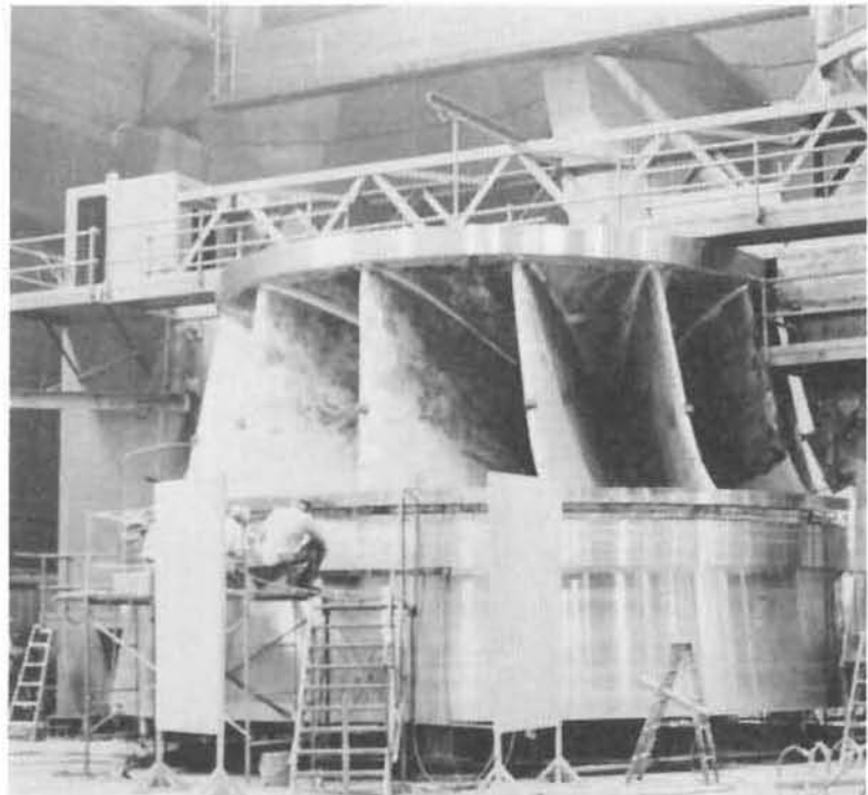
TURBINE RUNNER being machined at Grand Coulee project will produce about one million horsepower.
