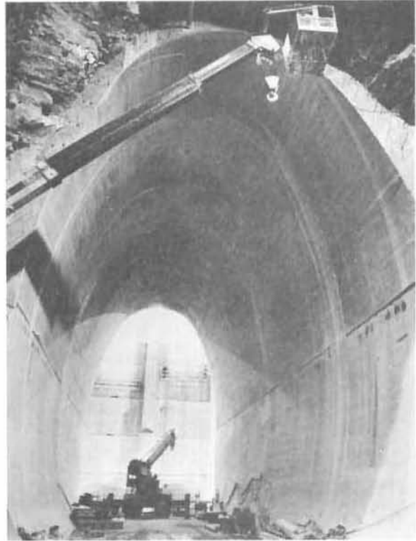
DRAFT TUBE and gate chamber under construction at Mica powerhouse.
