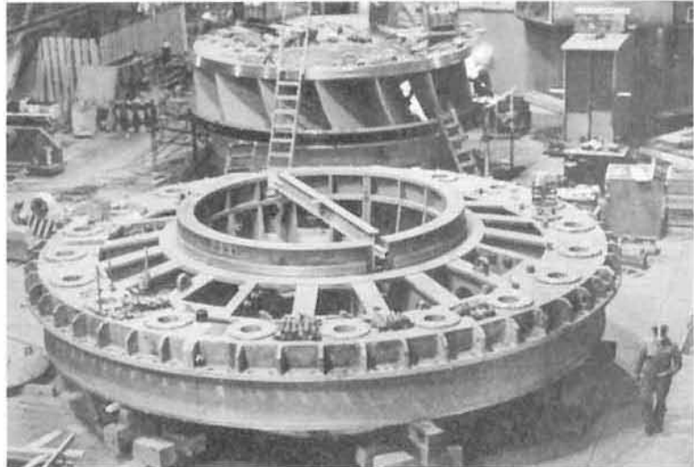
HEADCOVER for No. 4 turbine at Mica powerhouse.
