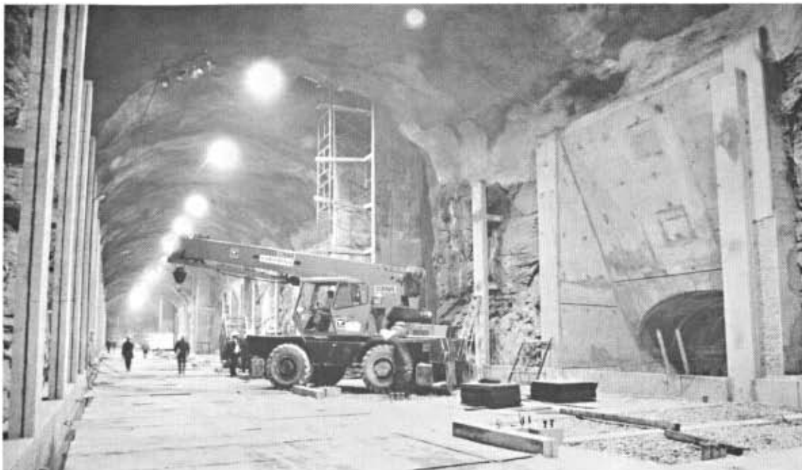
TRANSFORMER CHAMBER underground at Mica powerhouse.
