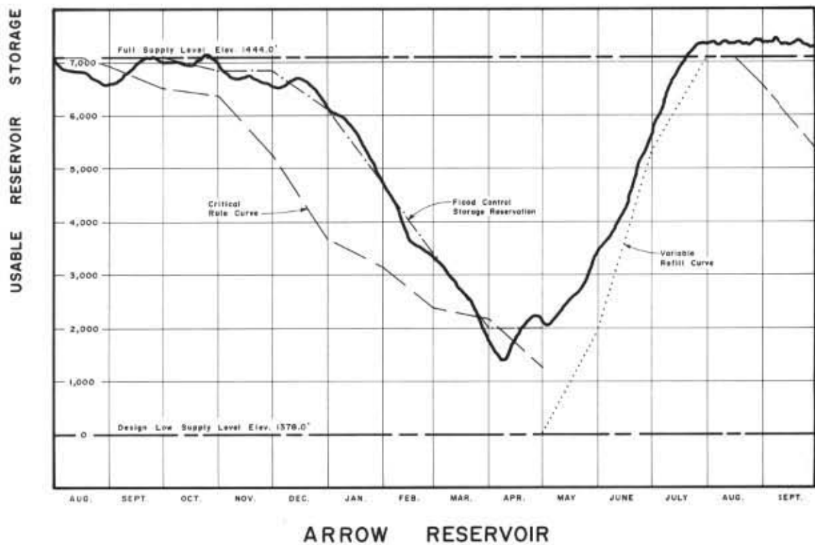
HYDROGRAPHS — Libby and Arrow reservoir levels for the 14-month period ending 30 September 1976.
