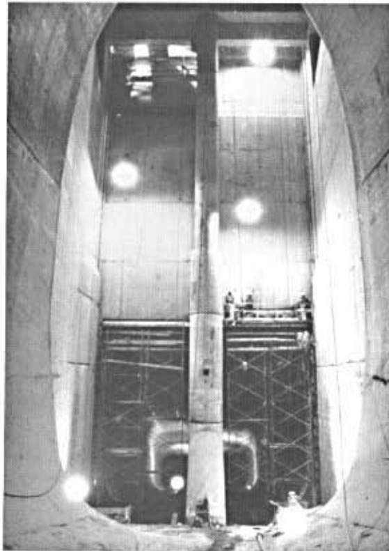
DRAFT TUBE GATES being installed for Unit No. 1 at Mica powerhouse.
