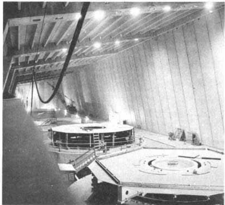
LIBBY POWERHOUSE interior.
