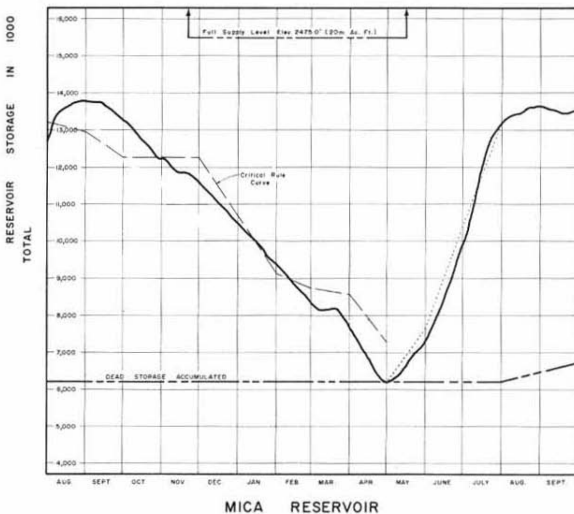
HYDROGRAPHS – Duncan and Mica reservoir levels for the 14-month period ending 30 September 1975.
