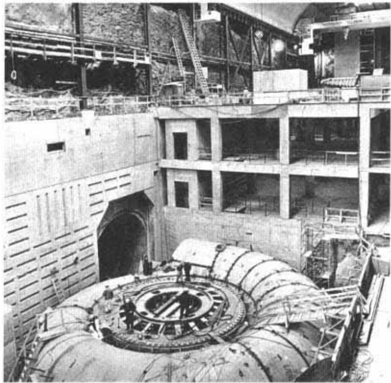
SCROLL CASE for Unit No. 1 at Mica powerhouse.
