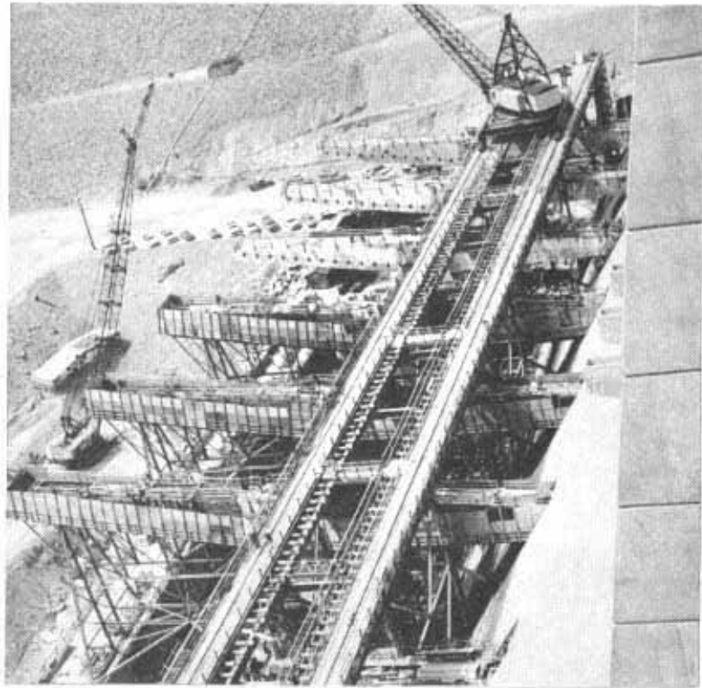
LIBBY POWERHOUSE construction seen from top of dam. May 1974.
