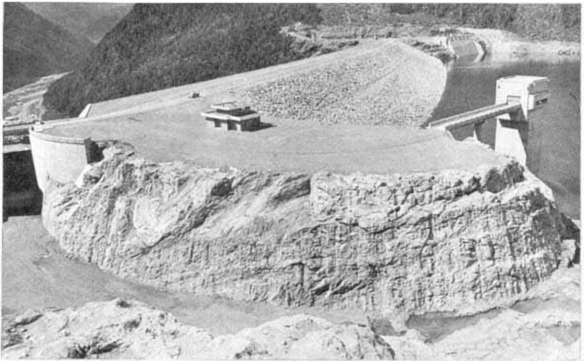
MICA DAM and intake works completed. July 1974.
