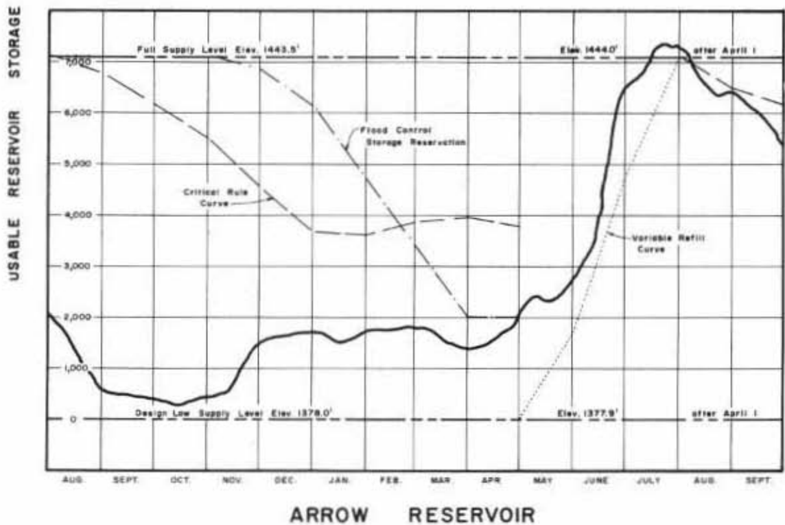
HYDROGRAPHS - Libby and Arrow reservoir levels for the 14-month period ending 30 September 1974.
