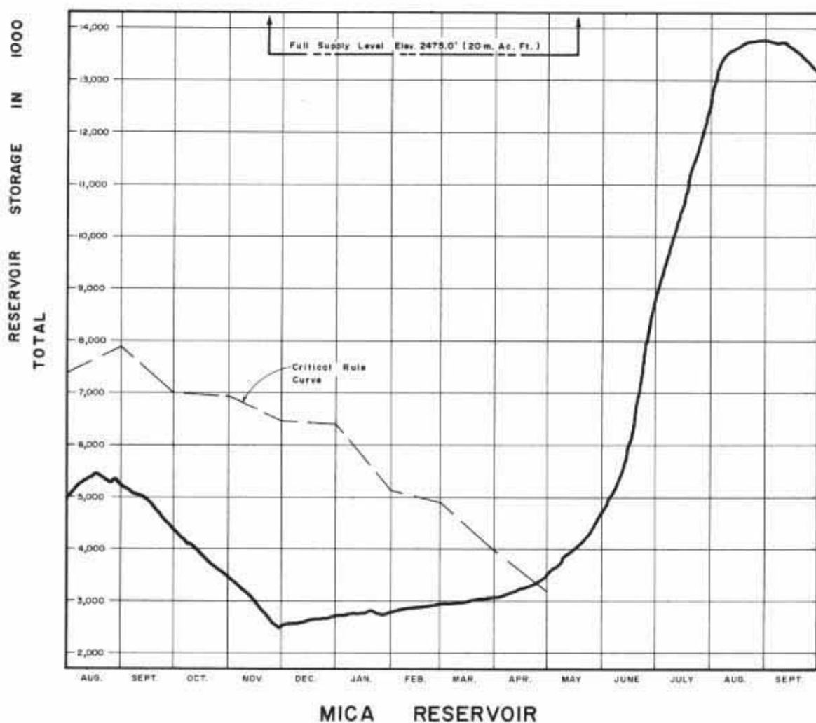
HYDROGRAPHS - Duncan and Mica reservoir levels for the 14-month period ending 30 September 1974.
