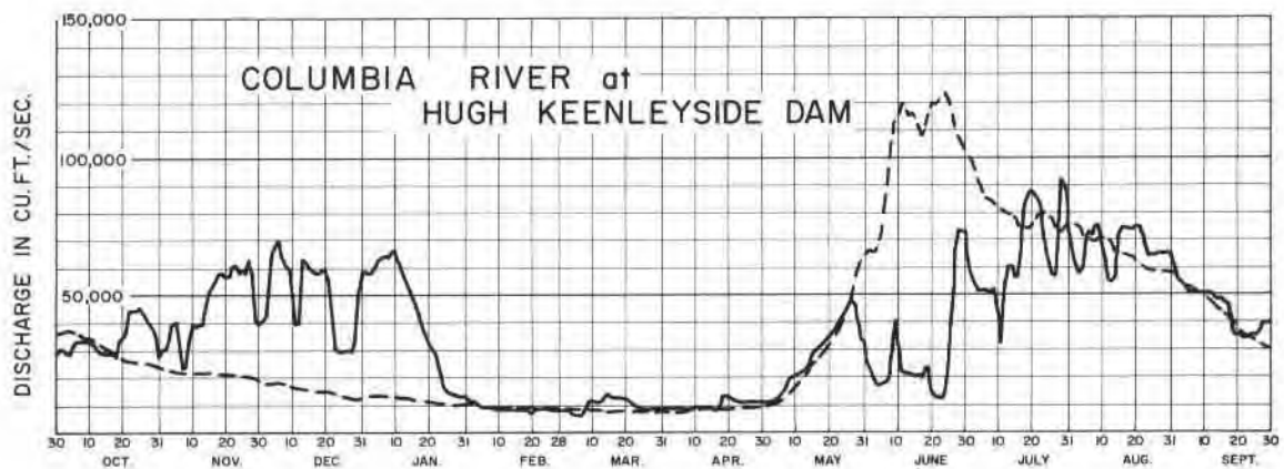
HYDROGRAPHS — Observed and Pre-Project flows for the year ending 30 September 1970.
